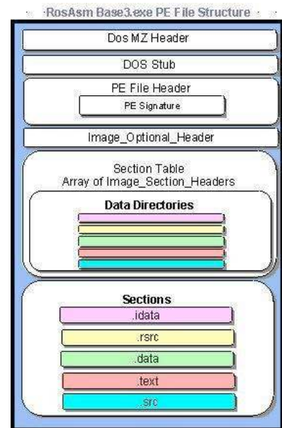
Figure 1: Structure of a PE File
